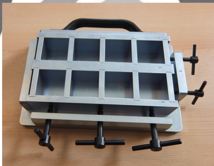
Eightfold mould 50x50x50 mm
