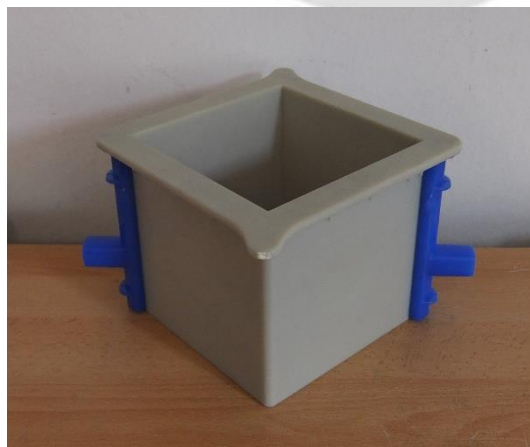
Plastic mould for cubes with two parts 150 mm
